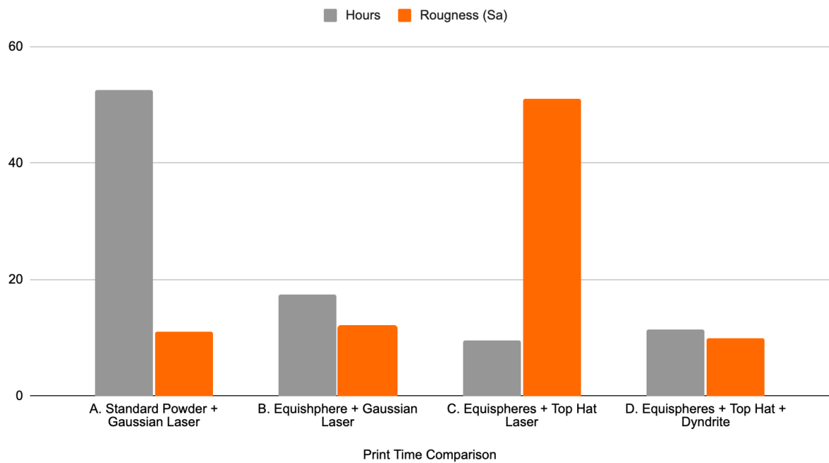
Chart 4: AconitySCAN Housing. Comparing print time and surface roughness (Sa).
