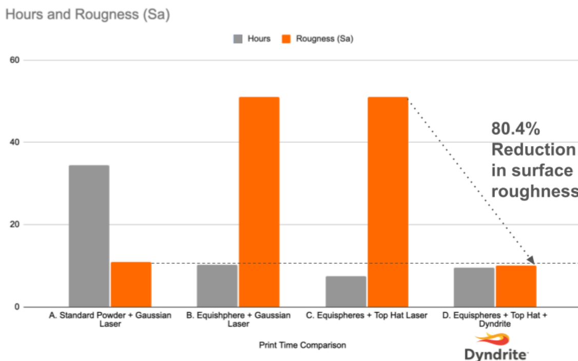
Chart 3: The addition of Dyndrite in Scenario D resulted in much improved surface finish without a significant increase in print time.
